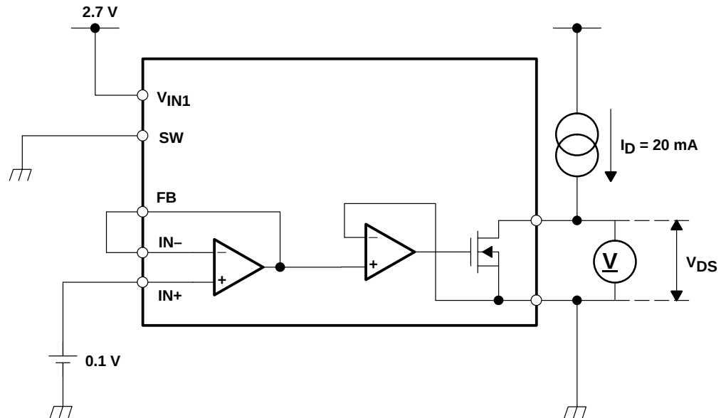
Figure 5. V_{OL}
